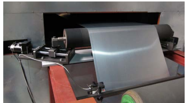
End Pivot Guider EPMP-TR(Single) is used on an Aluminum Web Finishing Machine
